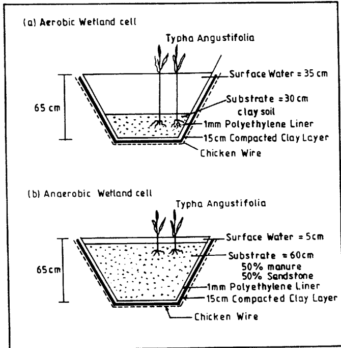
Figure 2 Typical design of aerobic and anaerobic wetland cells (Donahue, 1994)
