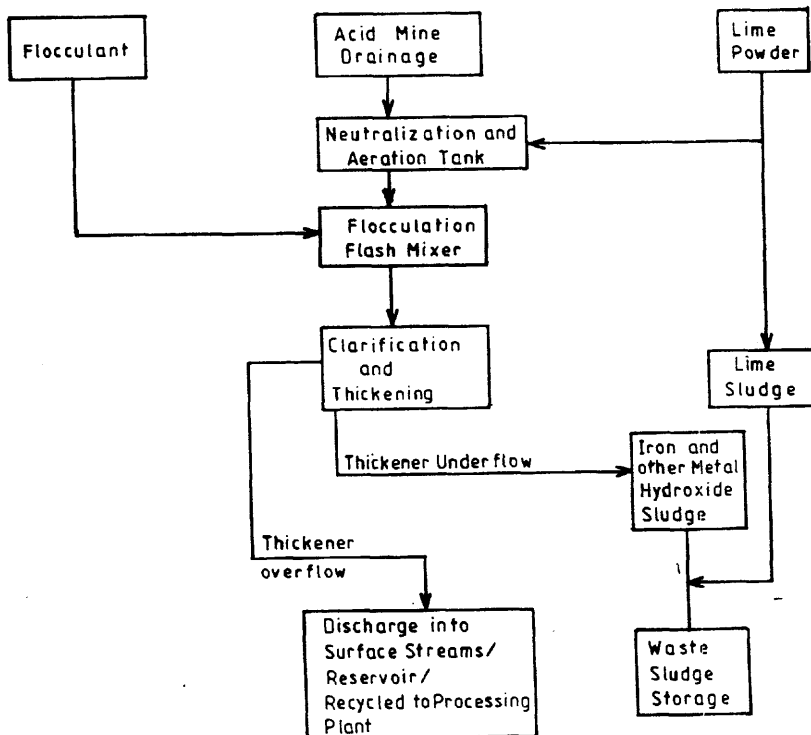
Figure 1. Block diagram for acid mine drainage treatment with lime
